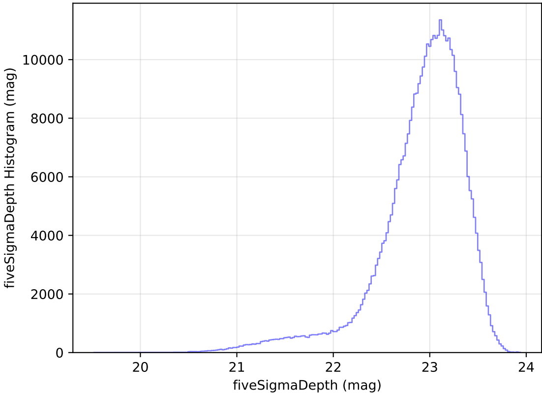
noroll_mjdp270_v3.4_10yrs WFD z band: fiveSigmaDepth Histogram
