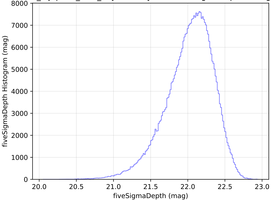
noroll_mjdp270_v3.4_10yrs WFD y band: fiveSigmaDepth Histogram
