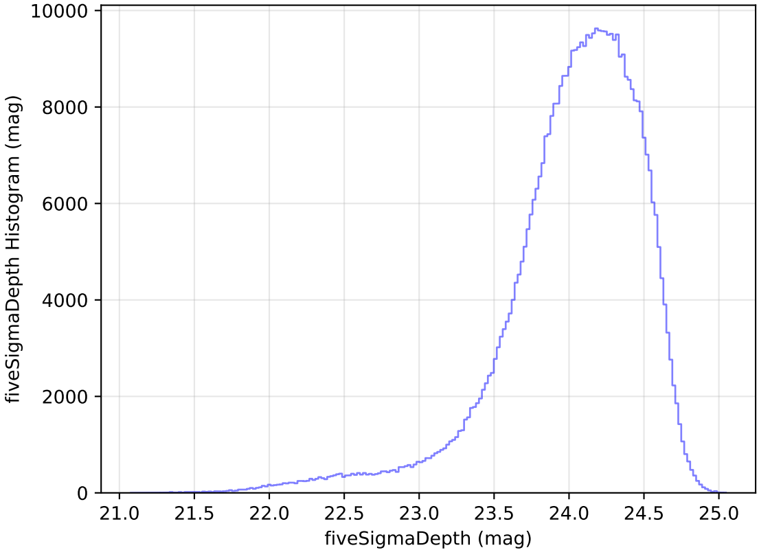
noroll_mjdp270_v3.4_10yrs WFD r band: fiveSigmaDepth Histogram
