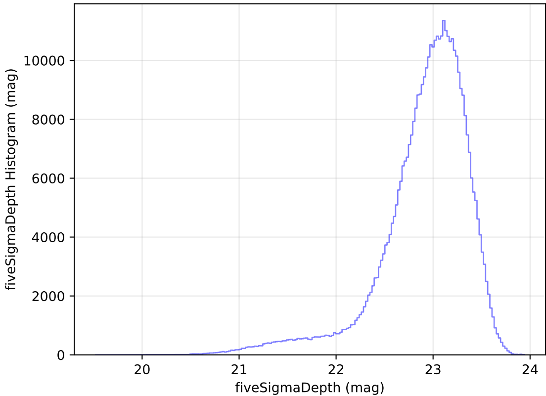
noroll_mjdp270_v3.4_10yrs All sky z band: fiveSigmaDepth Histogram
