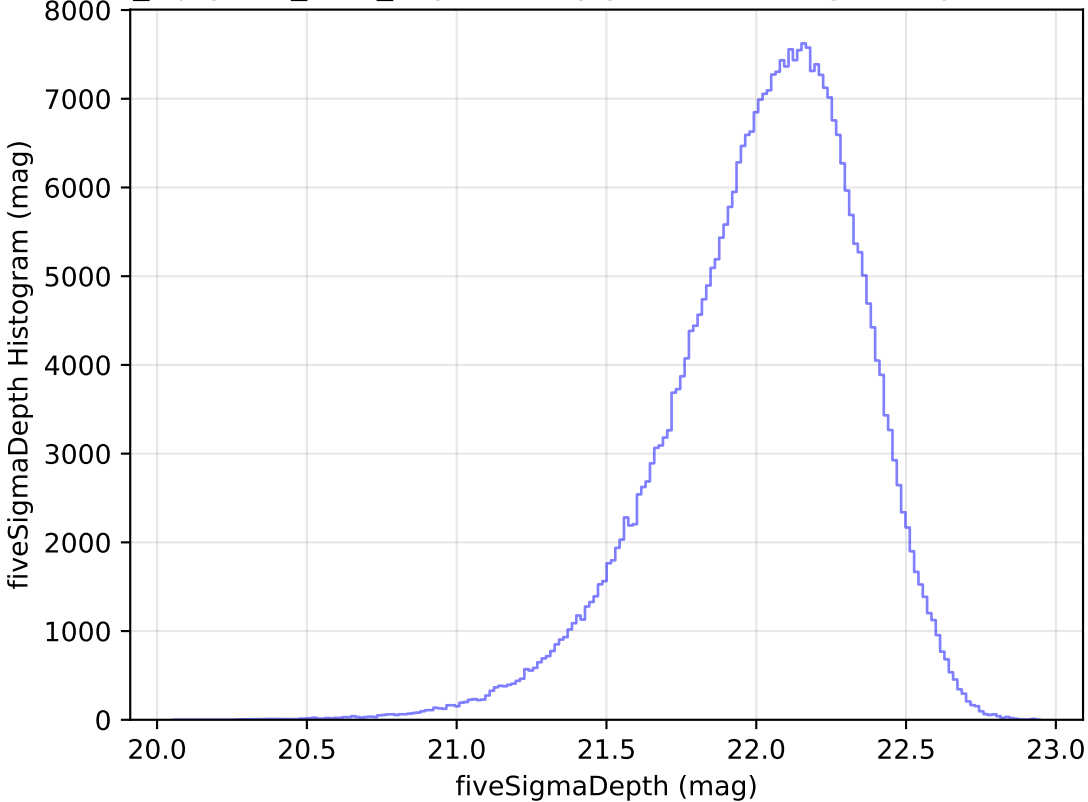
noroll_mjdp270_v3.4_10yrs All sky y band: fiveSigmaDepth Histogram
