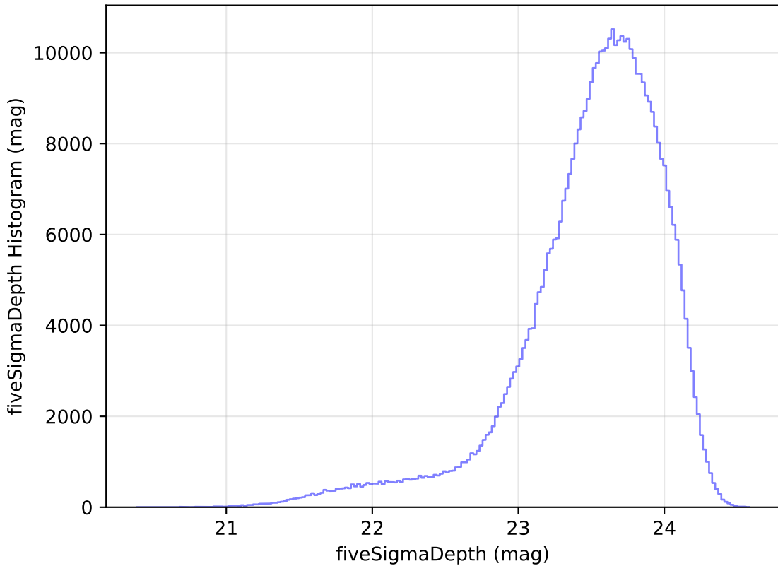
noroll_mjdp270_v3.4_10yrs All sky i band: fiveSigmaDepth Histogram
