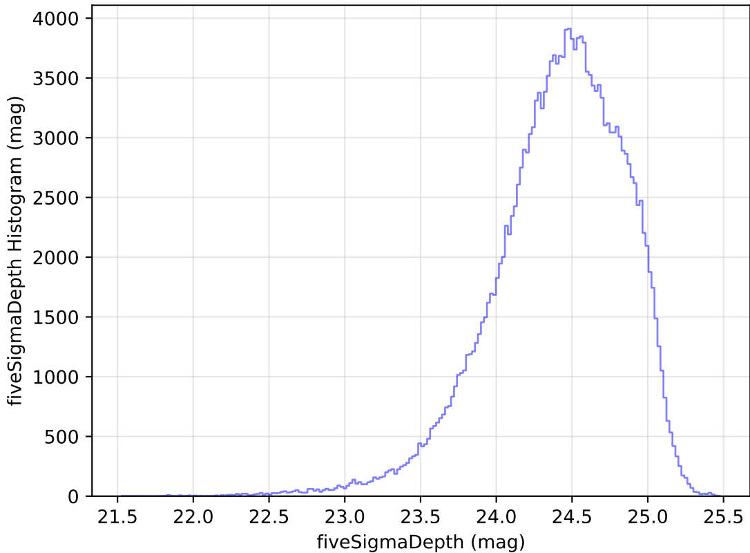
noroll_mjdp270_v3.4_10yrs All sky g band: fiveSigmaDepth Histogram
