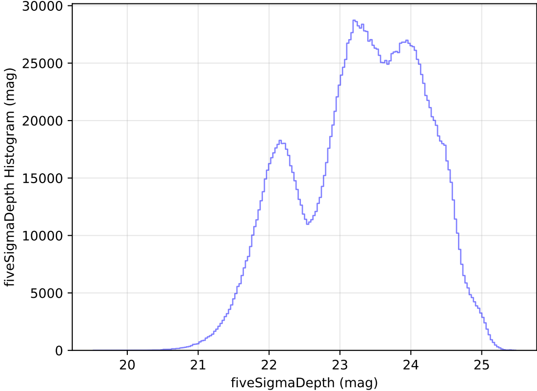
noroll_mjdp270_v3.4_10yrs All sky all bands: fiveSigmaDepth Histogram
