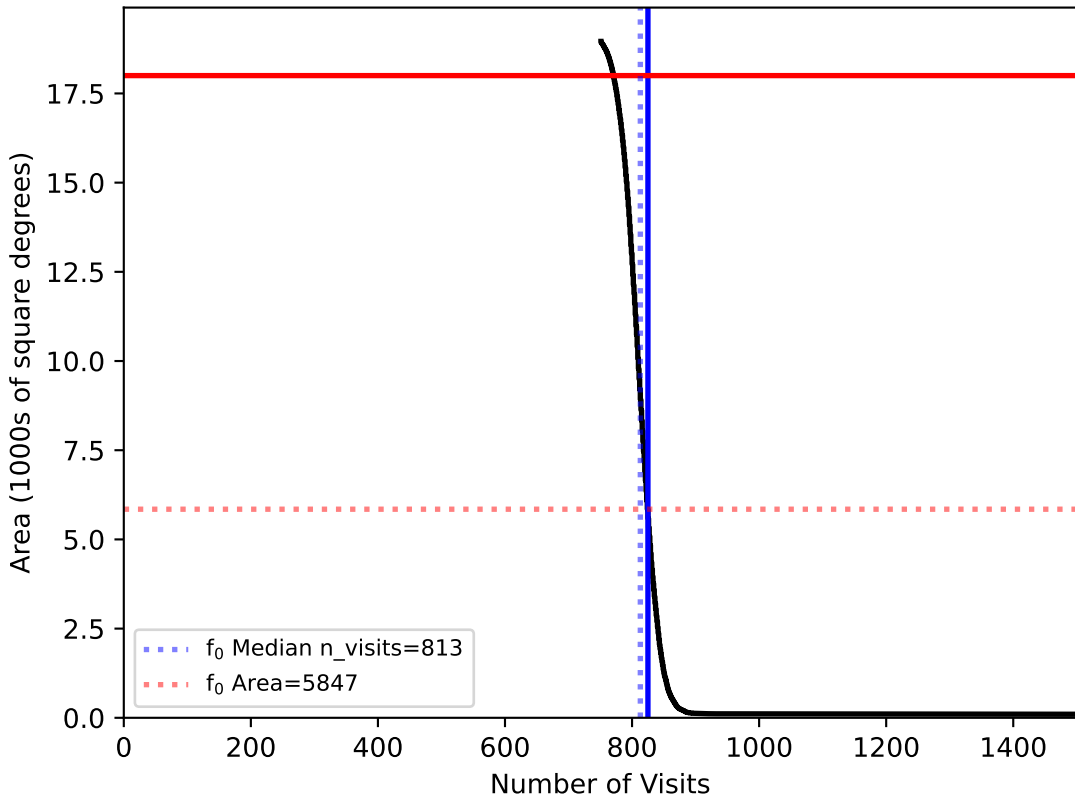
noroll_mjdp270_v3.4_10yrs WFD: f0
