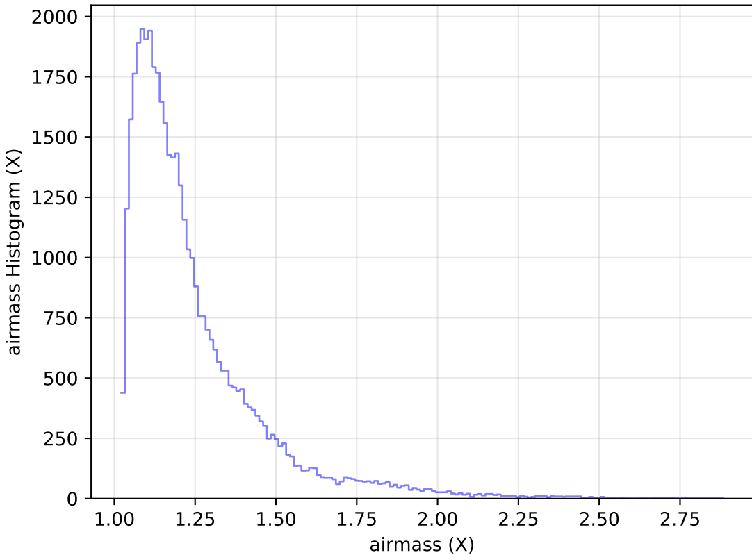
noroll_mjdp270_v3.4_10yrs Yr 1 y band: airmass Histogram
