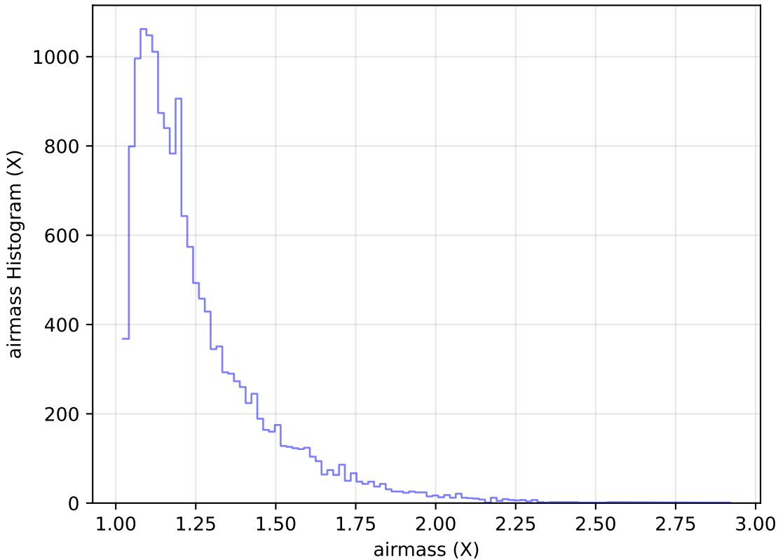
noroll_mjdp270_v3.4_10yrs Yr 1 u band: airmass Histogram
