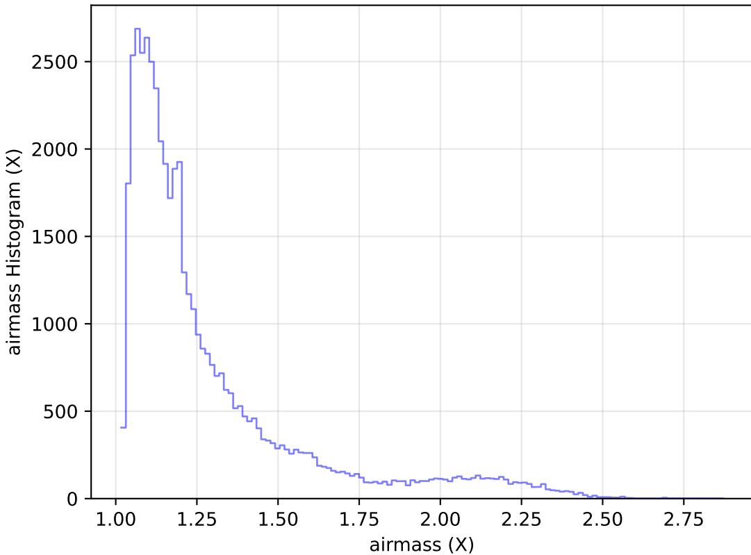
noroll_mjdp270_v3.4_10yrs Yr 1 r band: airmass Histogram
