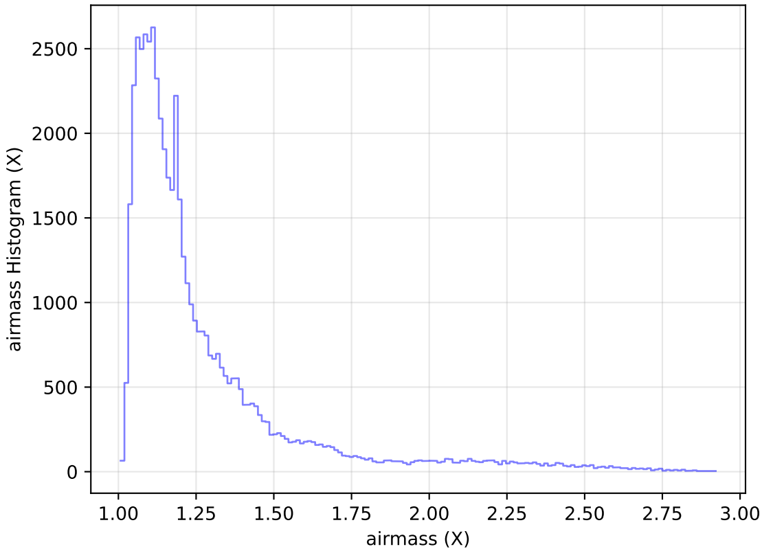
noroll_mjdp270_v3.4_10yrs Yr 1 i band: airmass Histogram
