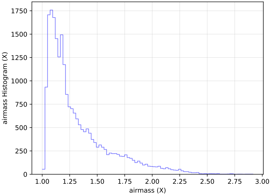
noroll_mjdp270_v3.4_10yrs Yr 1 g band: airmass Histogram
