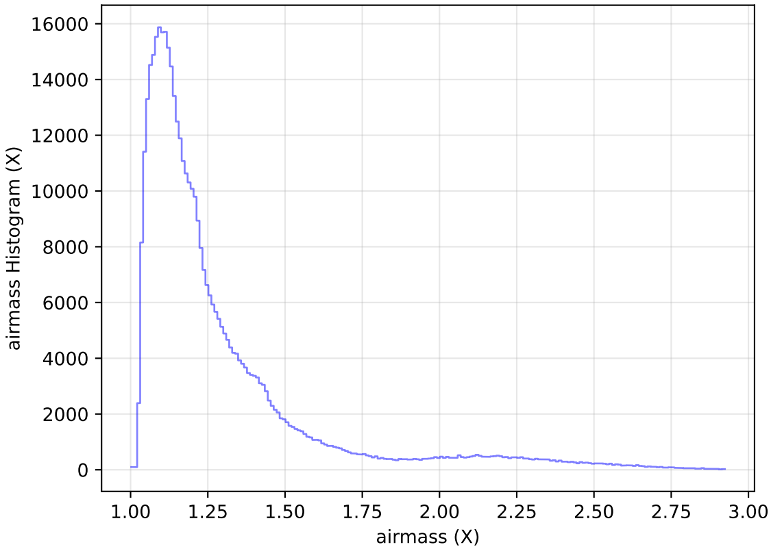
noroll_mjdp270_v3.4_10yrs WFD z band: airmass Histogram
