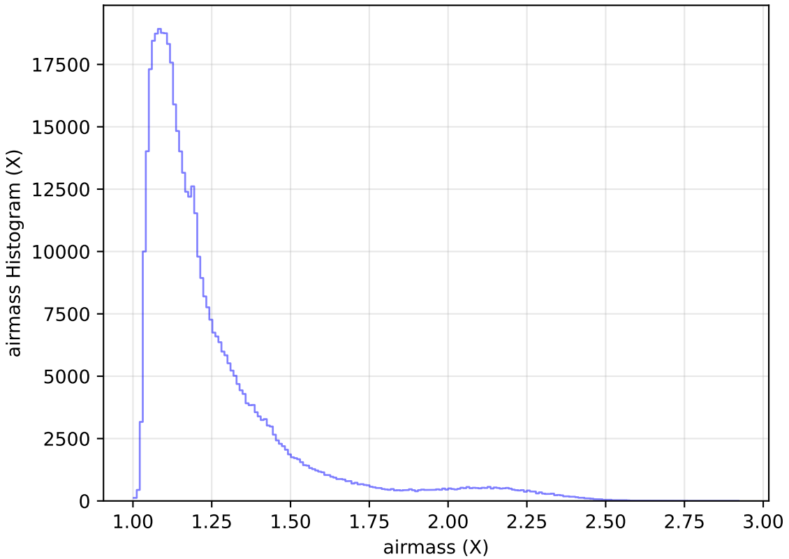
noroll_mjdp270_v3.4_10yrs WFD r band: airmass Histogram
