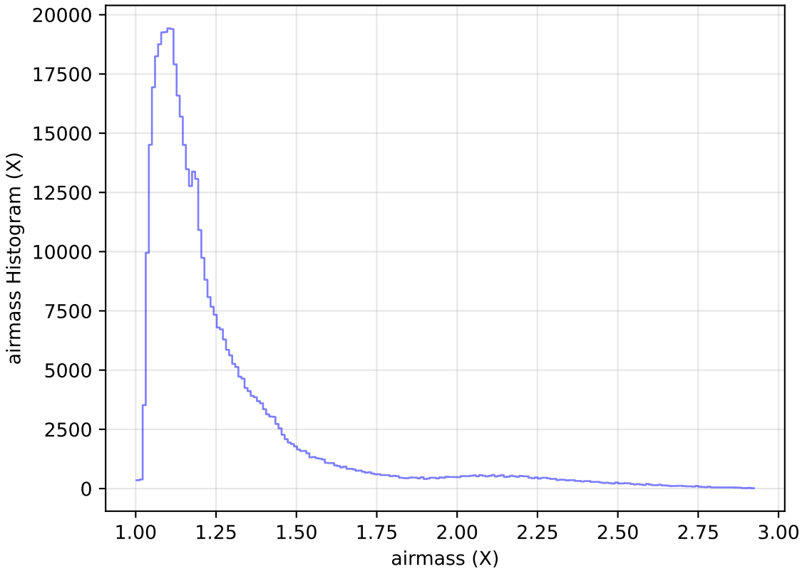
noroll_mjdp270_v3.4_10yrs WFD i band: airmass Histogram
