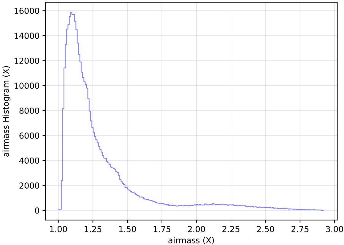
noroll_mjdp270_v3.4_10yrs All sky z band: airmass Histogram
