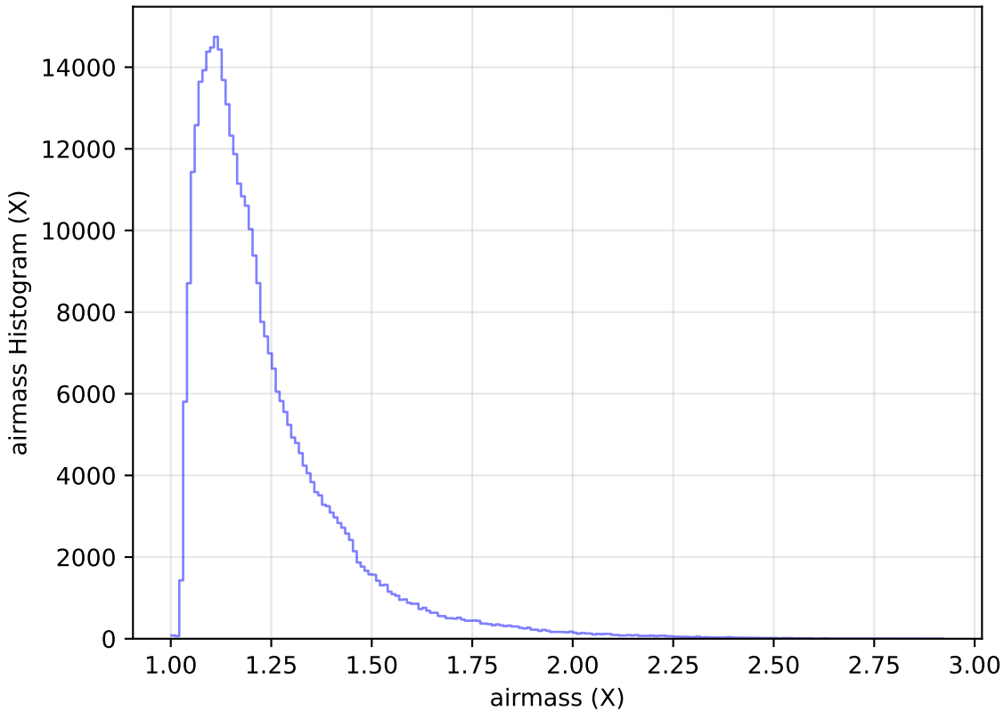
noroll_mjdp270_v3.4_10yrs All sky y band: airmass Histogram
