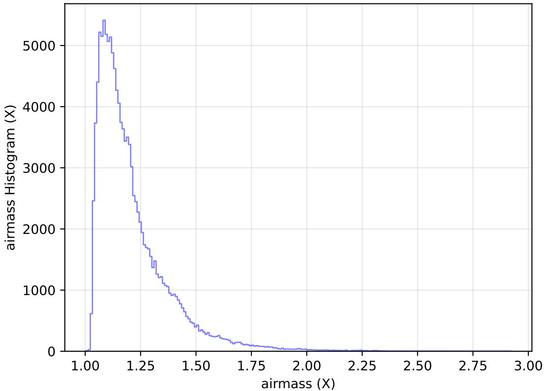
noroll_mjdp270_v3.4_10yrs All sky u band: airmass Histogram
