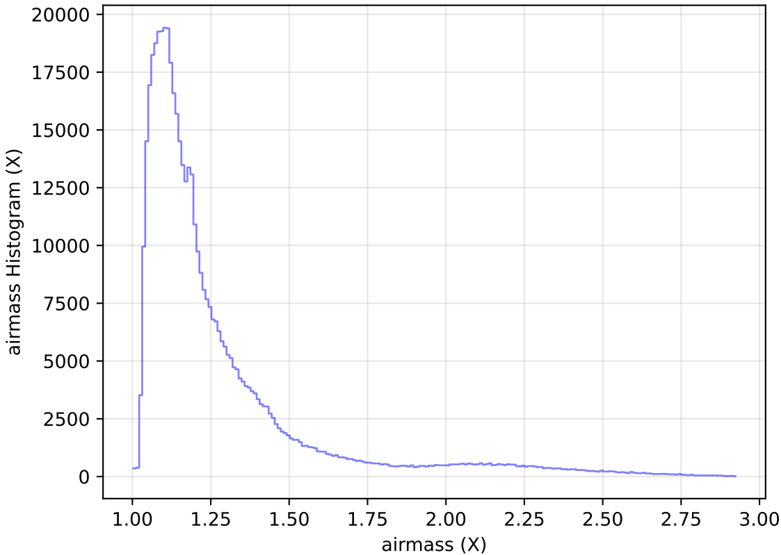
noroll_mjdp270_v3.4_10yrs All sky i band: airmass Histogram
