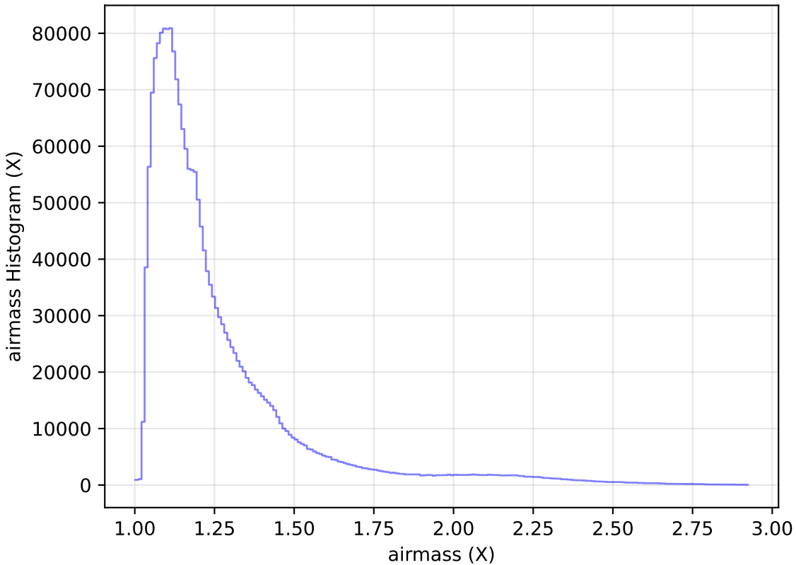
noroll_mjdp270_v3.4_10yrs All sky all bands: airmass Histogram
