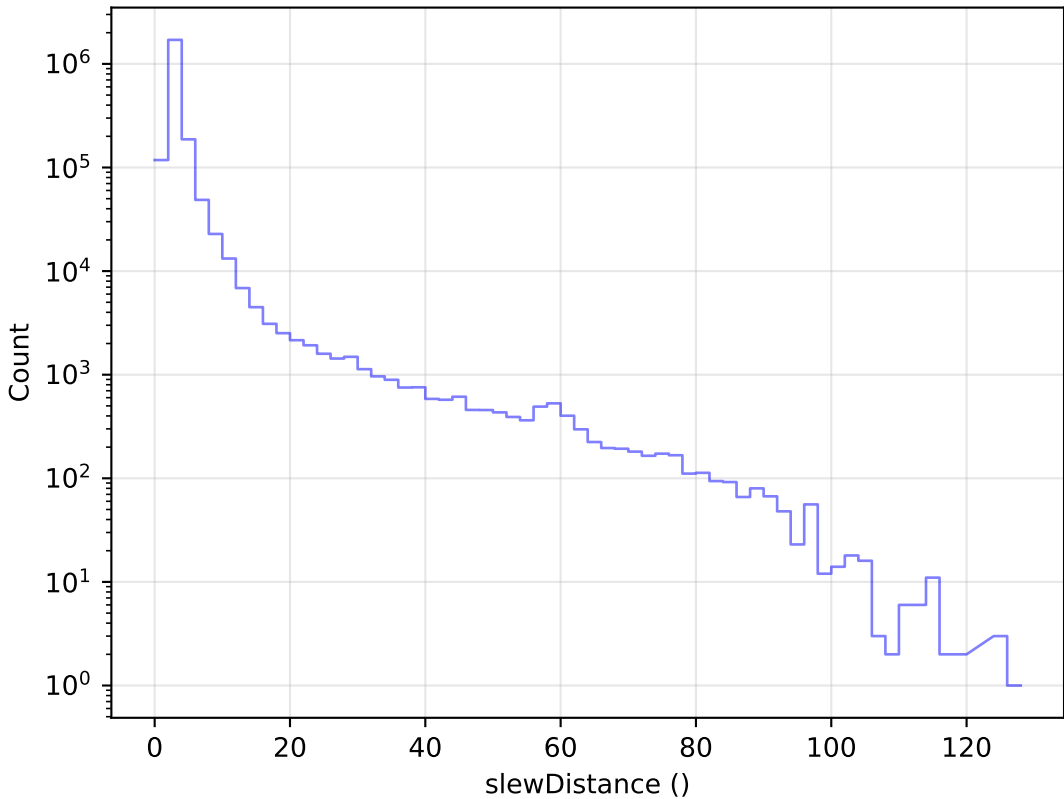
noroll_mjdp270_v3.4_10yrs All visits: Slew Distance Histogram
