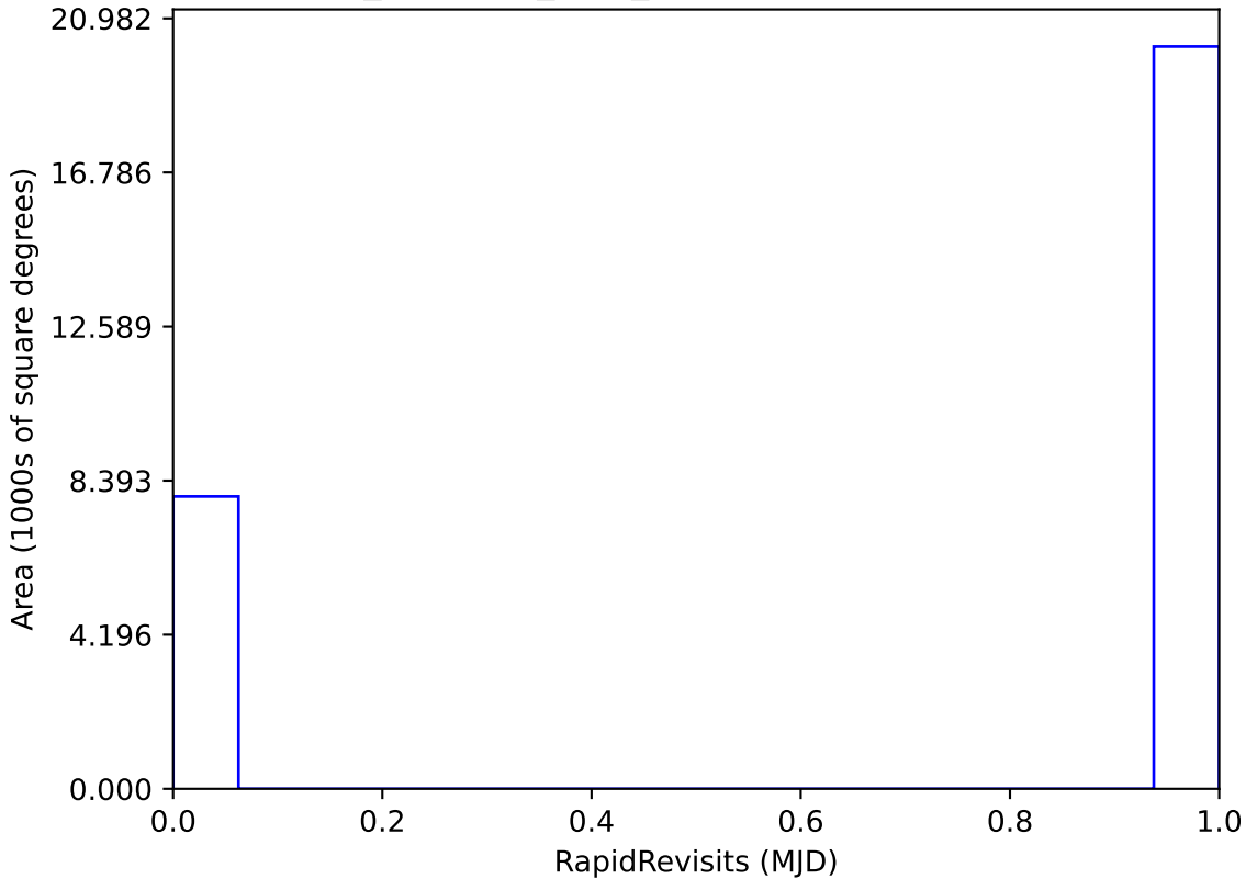
noroll_mjdp270_v3.4_10yrs All sky: RapidRevisits
