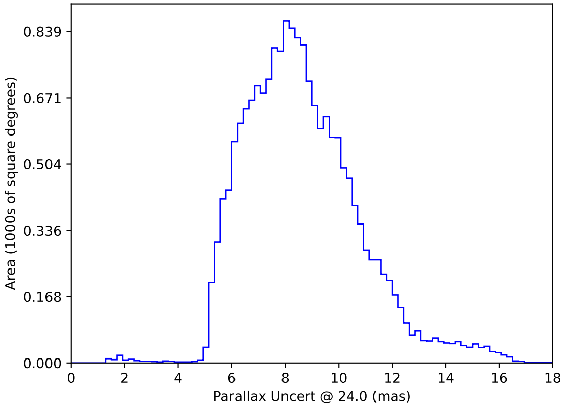
noroll_mjdp270_v3.4_10yrs WFD: Parallax Uncert @ 24.0
