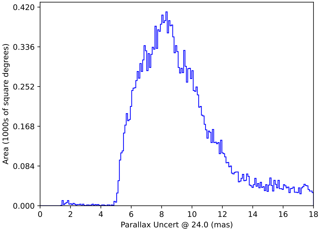
noroll_mjdp270_v3.4_10yrs All sky: Parallax Uncert @ 24.0
