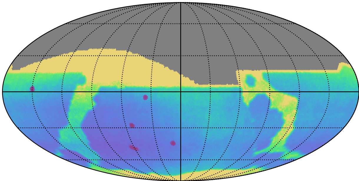
noroll_mjdp270_v3.4_10yrs All sky: Parallax Uncert @ 22.4
