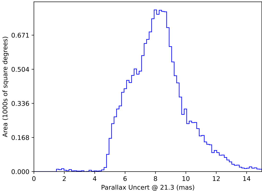
noroll_mjdp270_v3.4_10yrs WFD y band only: Parallax Uncert @ 21.3
