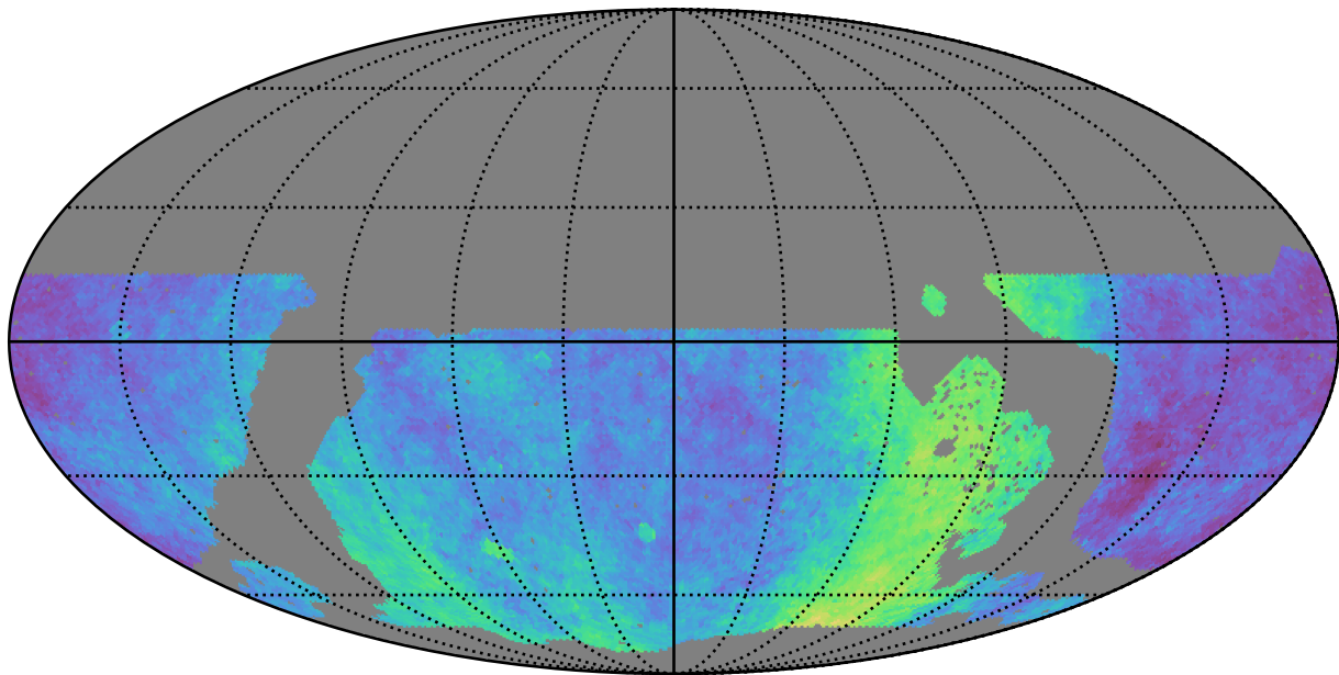
noroll_mjdp270_v3.4_10yrs WFD: Parallax Coverage @ 24.0
