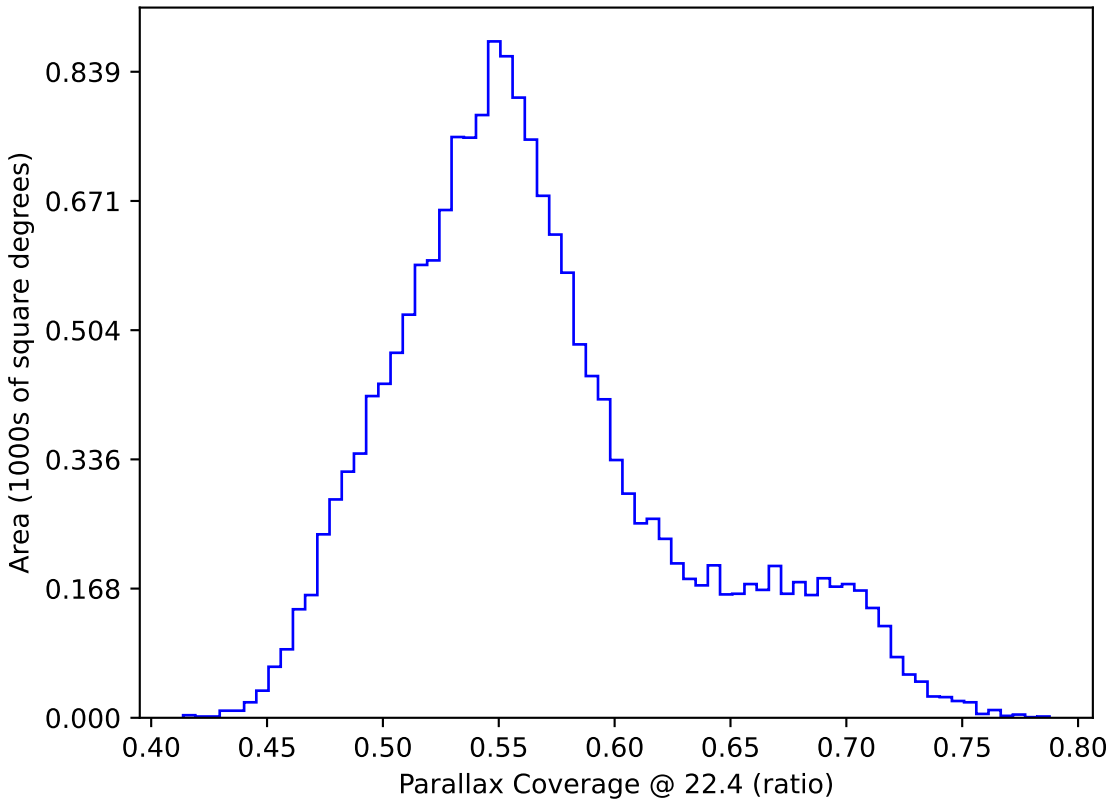
noroll_mjdp270_v3.4_10yrs WFD: Parallax Coverage @ 22.4
