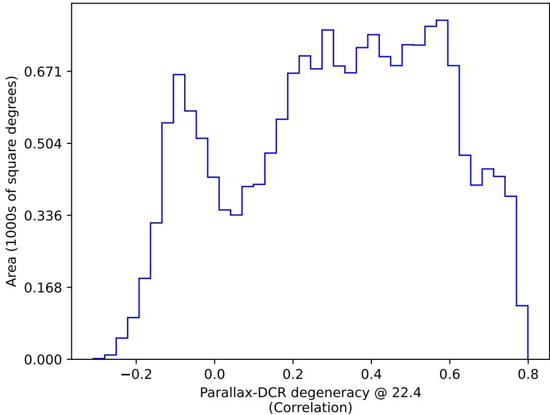
noroll_mjdp270_v3.4_10yrs WFD: Parallax-DCR degeneracy @ 22.4
