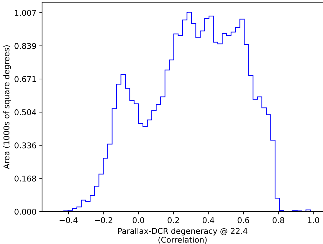
noroll_mjdp270_v3.4_10yrs All sky: Parallax-DCR degeneracy @ 22.4
