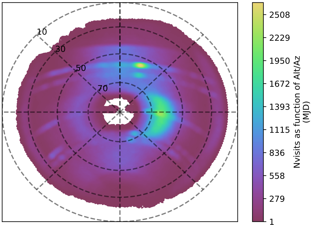
noroll_mjdp270_v3.4_10yrs z band: Nvisits as function of Alt/Az
