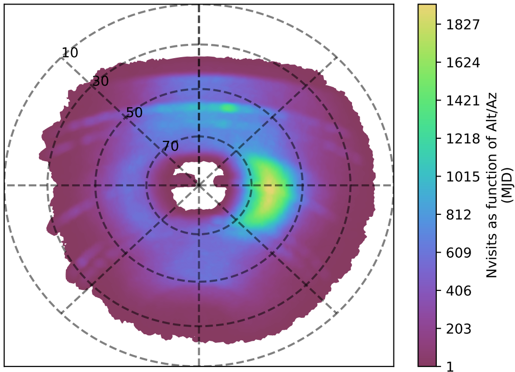
noroll_mjdp270_v3.4_10yrs y band: Nvisits as function of Alt/Az
