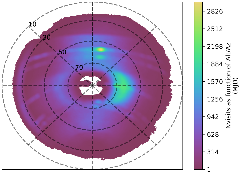
noroll_mjdp270_v3.4_10yrs r band: Nvisits as function of Alt/Az
