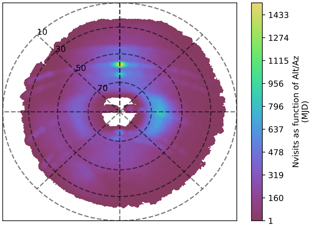
noroll_mjdp270_v3.4_10yrs g band: Nvisits as function of Alt/Az
