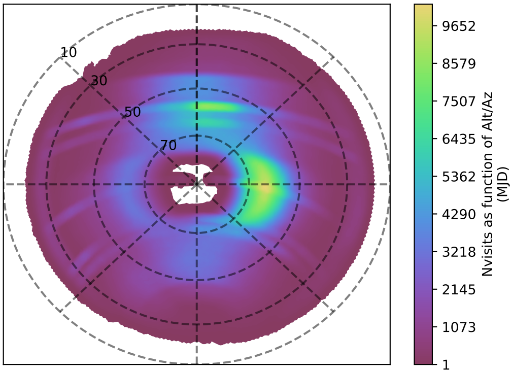
noroll_mjdp270_v3.4_10yrs all bands: Nvisits as function of Alt/Az
