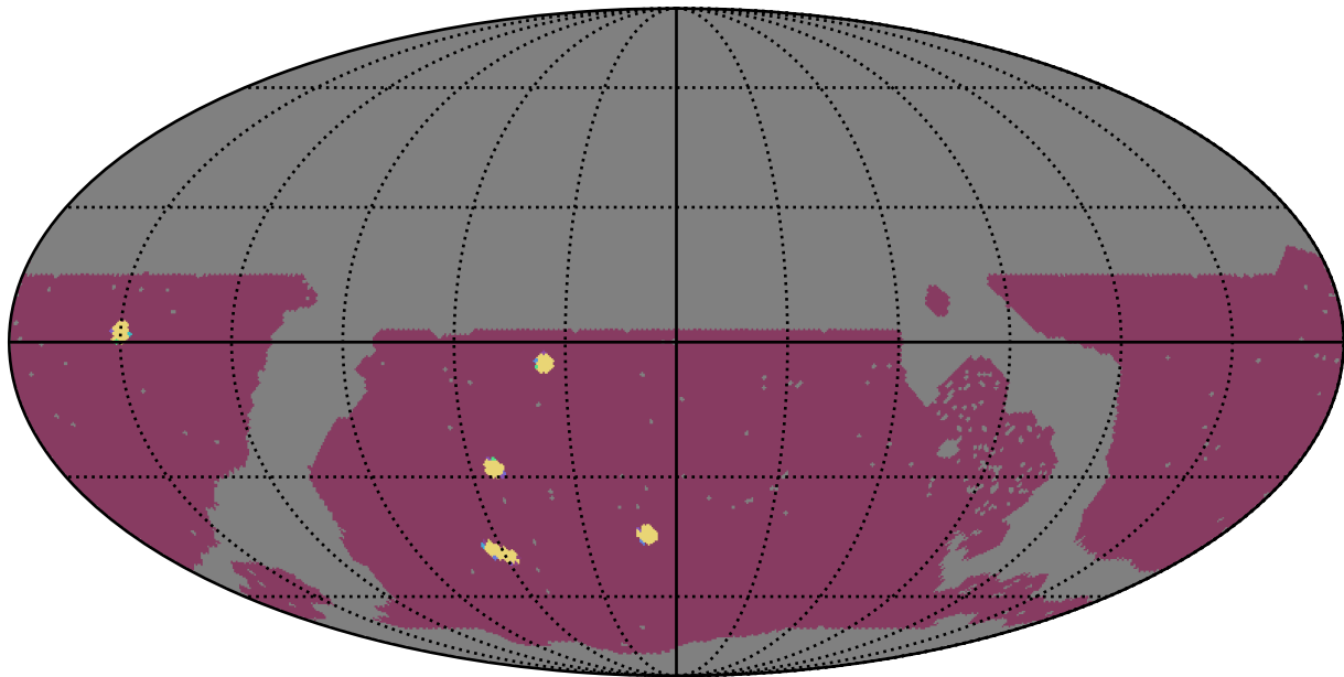
noroll_mjdp270_v3.4_10yrs WFD: NumberOfQuickRevisits
