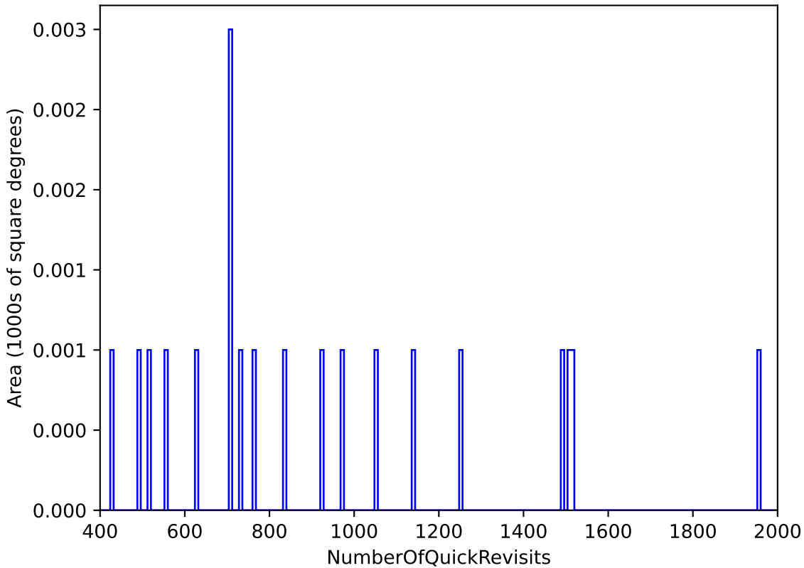
noroll_mjdp270_v3.4_10yrs WFD: NumberOfQuickRevisits
