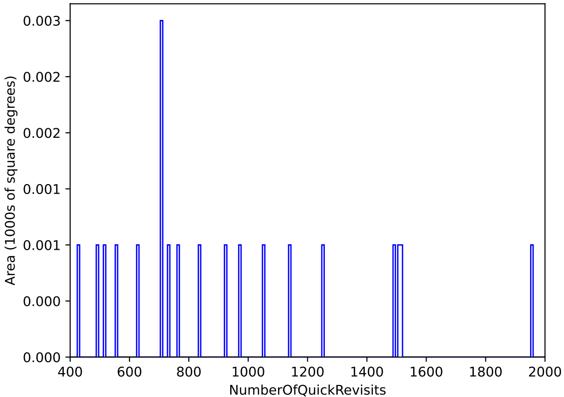
noroll_mjdp270_v3.4_10yrs All sky: NumberOfQuickRevisits
