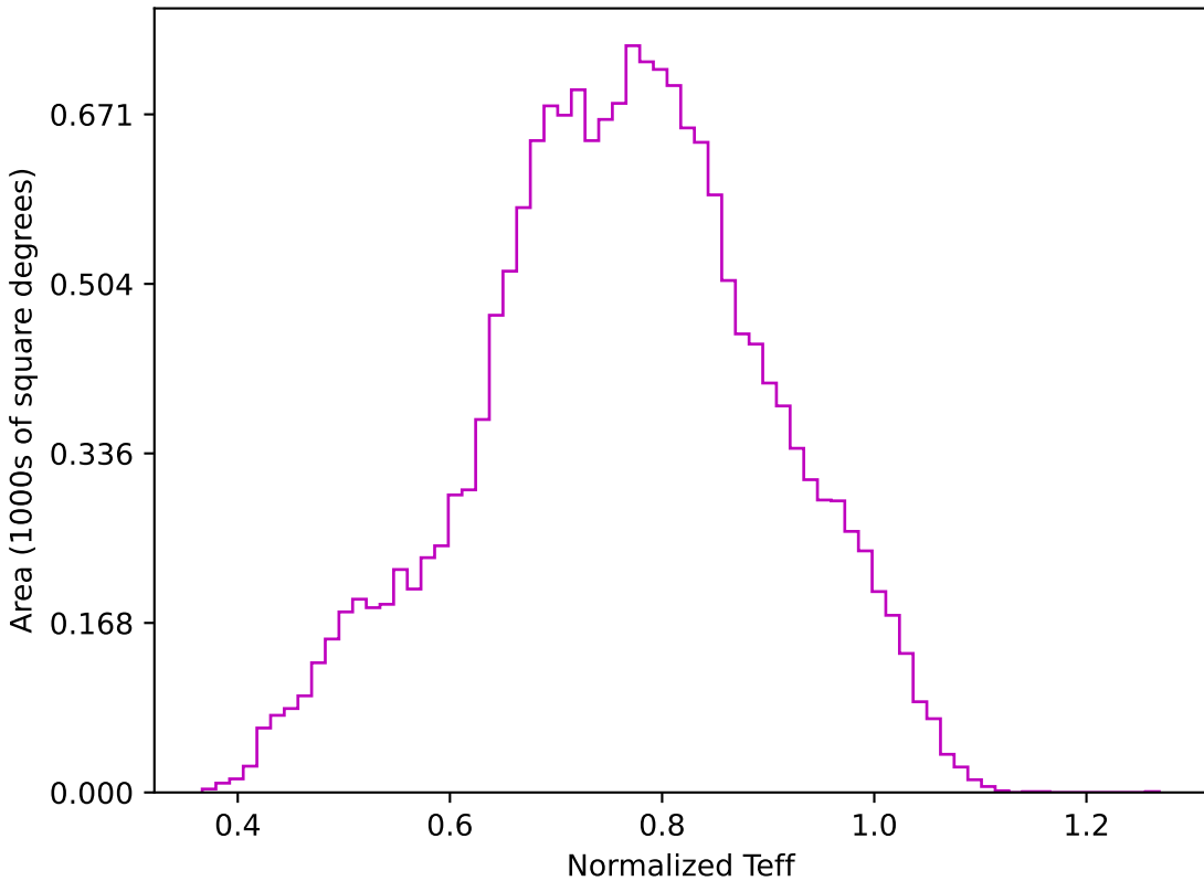
noroll_mjdp270_v3.4_10yrs WFD z band: Normalized Teff
