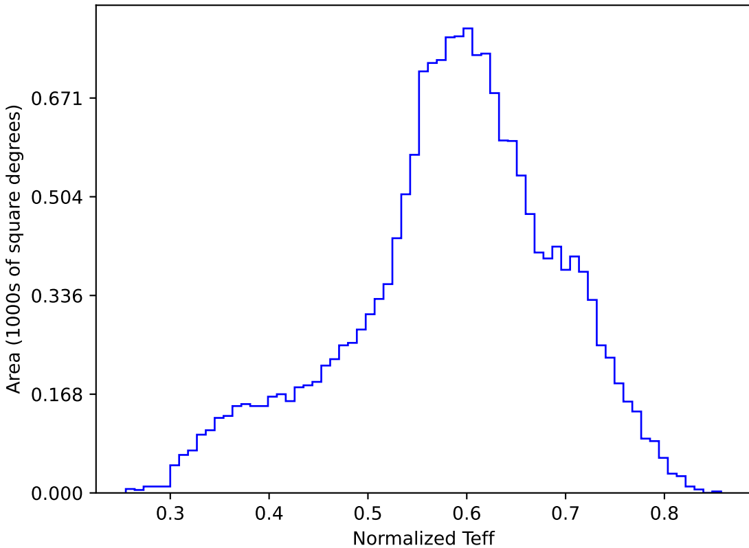
noroll_mjdp270_v3.4_10yrs WFD y band: Normalized Teff
