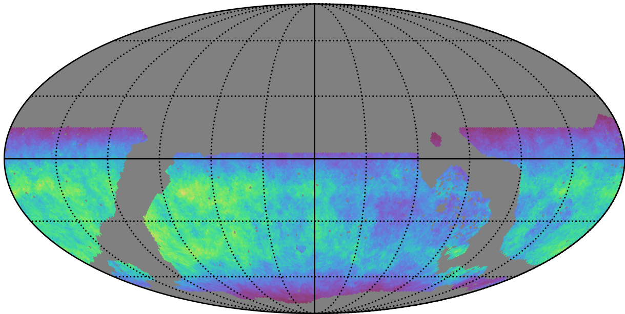
noroll_mjdp270_v3.4_10yrs WFD u band: Normalized Teff
