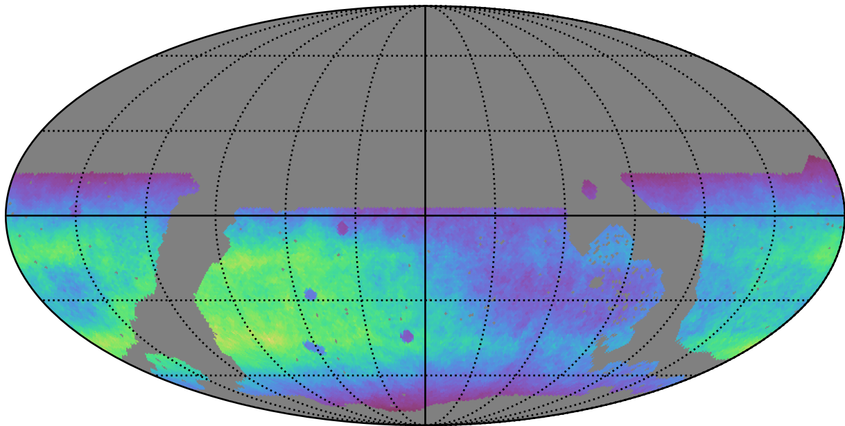
noroll_mjdp270_v3.4_10yrs WFD r band: Normalized Teff
