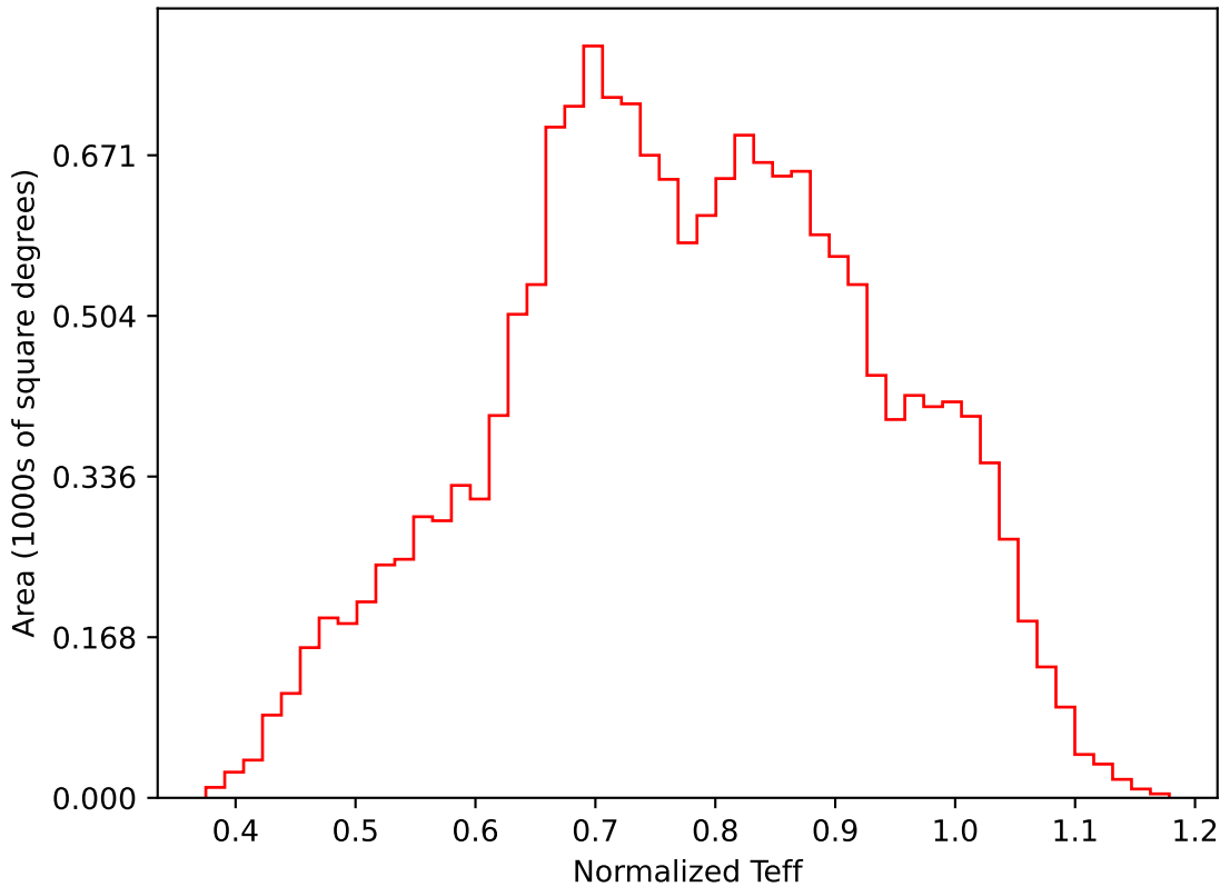
noroll_mjdp270_v3.4_10yrs WFD i band: Normalized Teff
