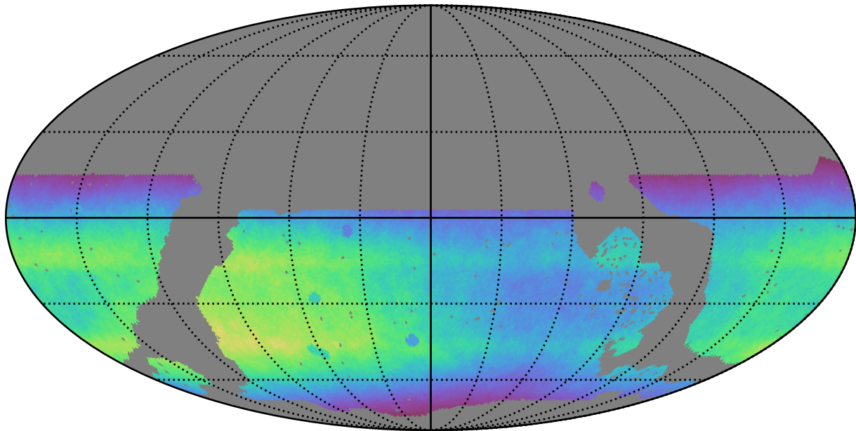
noroll_mjdp270_v3.4_10yrs WFD all bands: Normalized Teff
