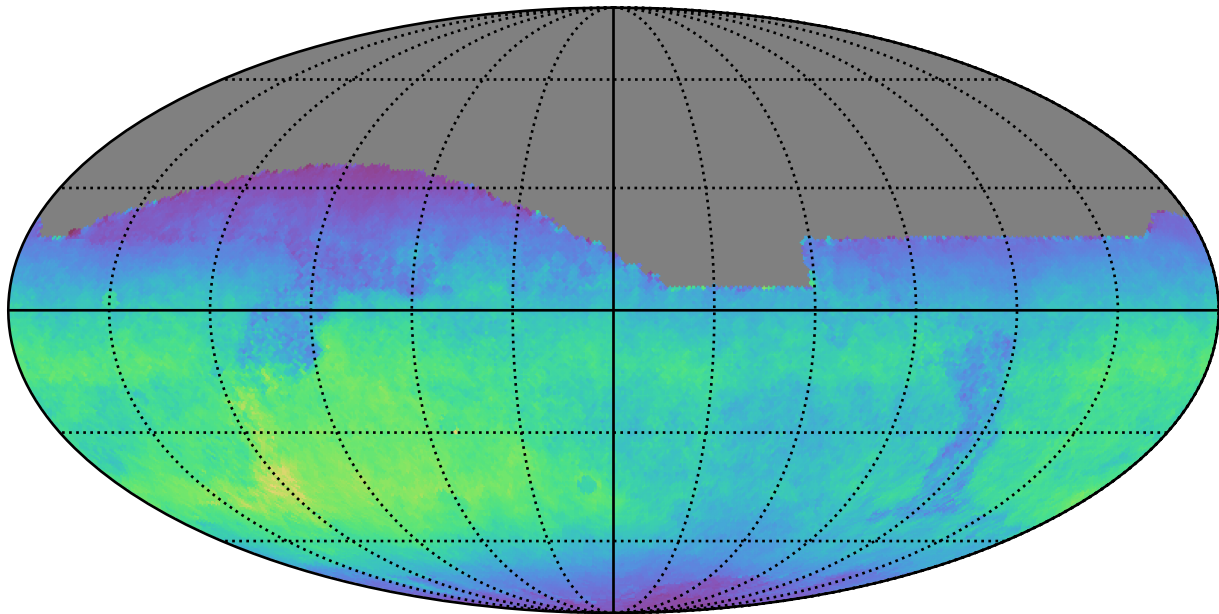
noroll_mjdp270_v3.4_10yrs All sky z band: Normalized Teff
