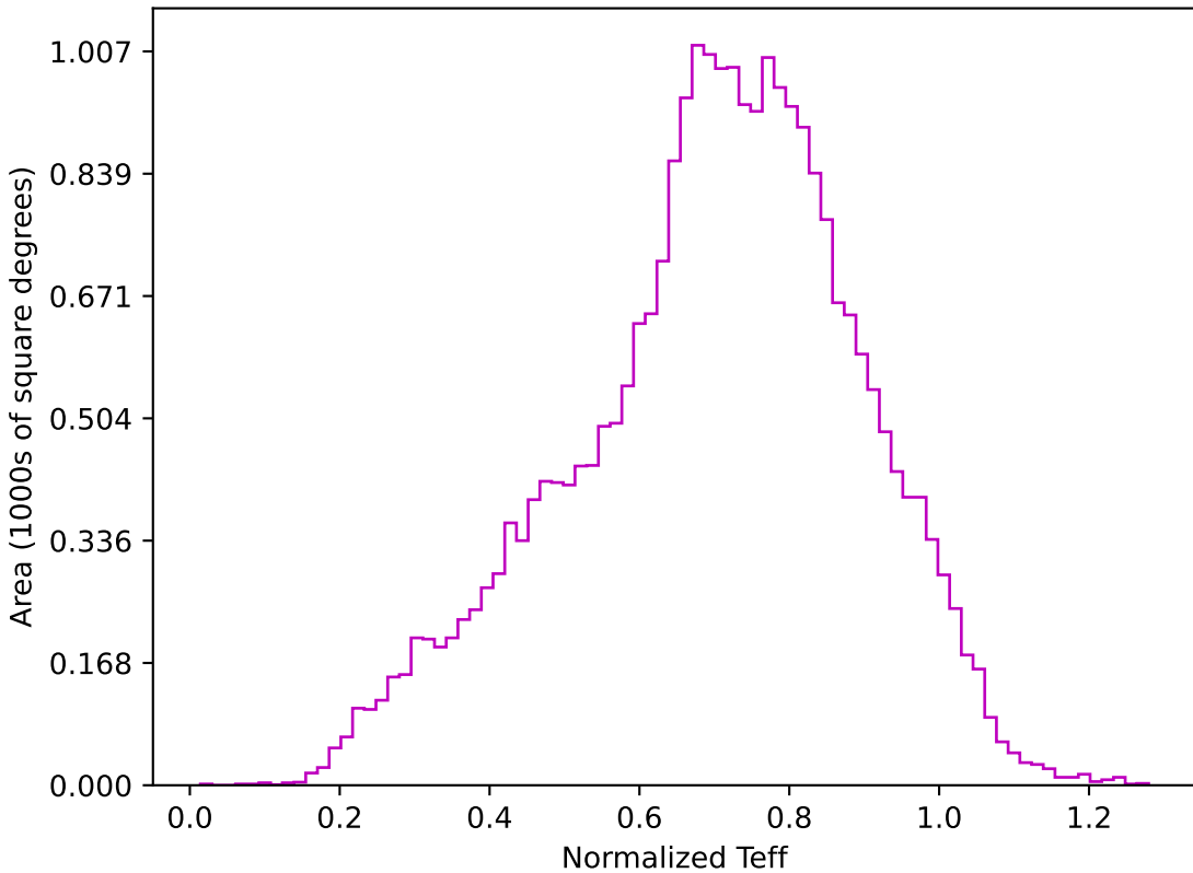
noroll_mjdp270_v3.4_10yrs All sky z band: Normalized Teff
