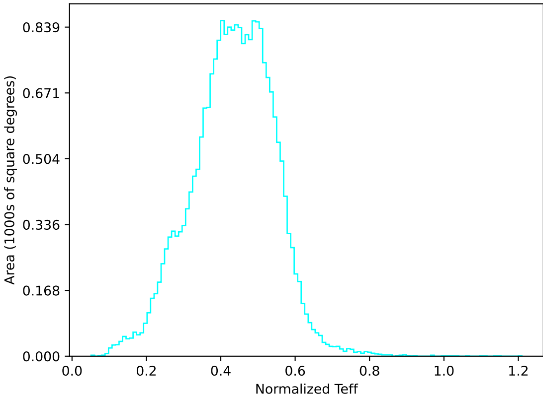
noroll_mjdp270_v3.4_10yrs All sky u band: Normalized Teff
