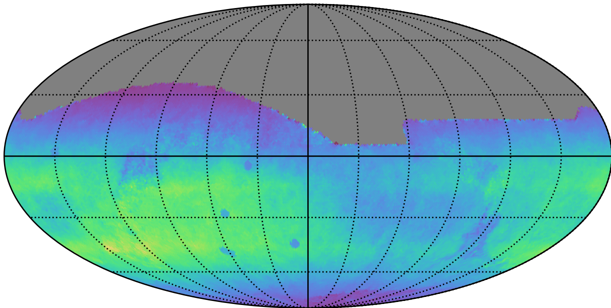
noroll_mjdp270_v3.4_10yrs All sky r band: Normalized Teff
